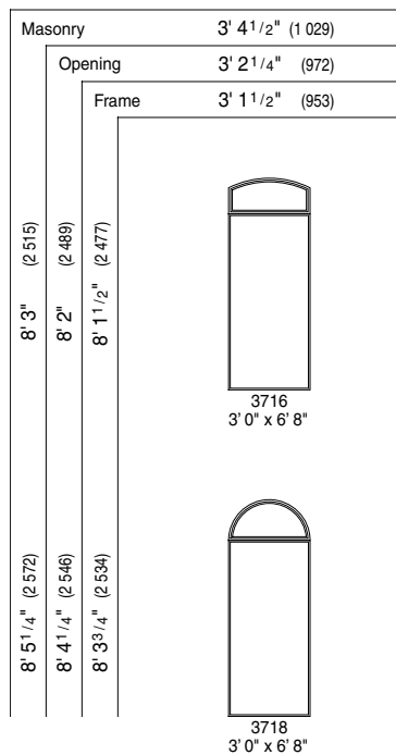
3' 0" x 6' 8" Out-Swing Doors with Circlehead & Arch Head Transoms
