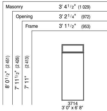
3' 0" x 6' 8" Out-Swing Doors with Transoms
