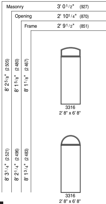
2' 8" x 6' 8" Out-Swing Doors with Circlehead & Arch Head Transoms
