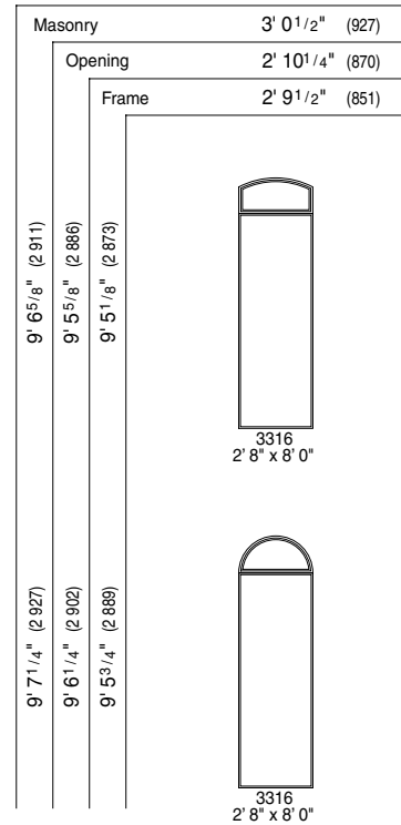
2' 8" x 8' 0" Out-Swing Doors with Circlehead & Arch Head Transoms
