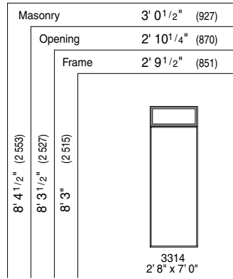
2' 8" x 7' 0" Out-Swing Doors with Transoms
