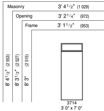
3' 0" x 7' 0" Out-Swing Doors with Transoms
