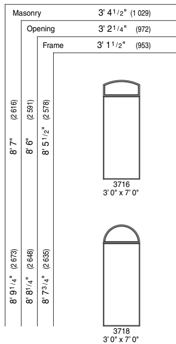
3' 0" x 7' 0" Out-Swing Doors with Circlehead & Arch Head Transoms
