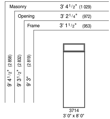
3' 0" x 8' 0" Out-Swing Doors with Transoms
