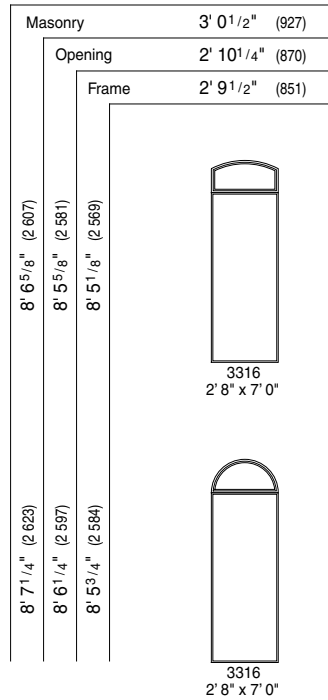
2' 8" x 7' 0" Out-Swing Doors with Circlehead & Arch Head Transoms
