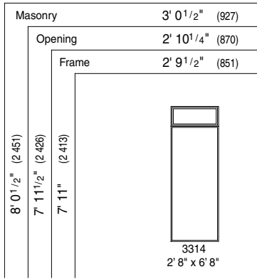
2' 8" x 6' 8" Out-Swing Doors with Transoms
