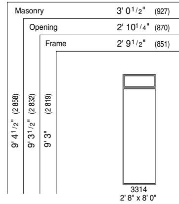
2' 8" x 8' 0" Out-Swing Doors with Transoms
