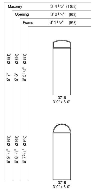
3' 0" x 8' 0" Out-Swing Doors with Circlehead & Arch Head Transoms
